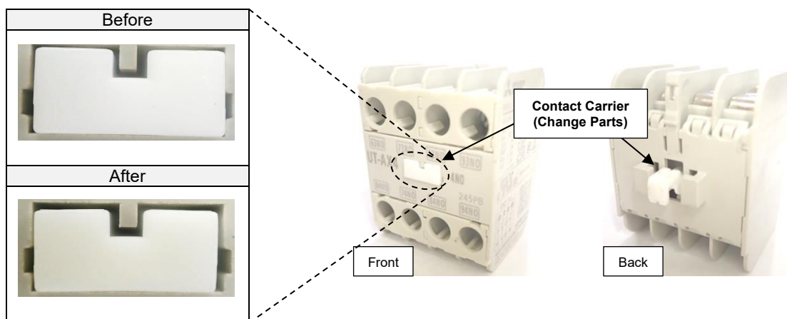
Fig. Appearance of the Applicable Model (Representative Model: UT-AX4)
