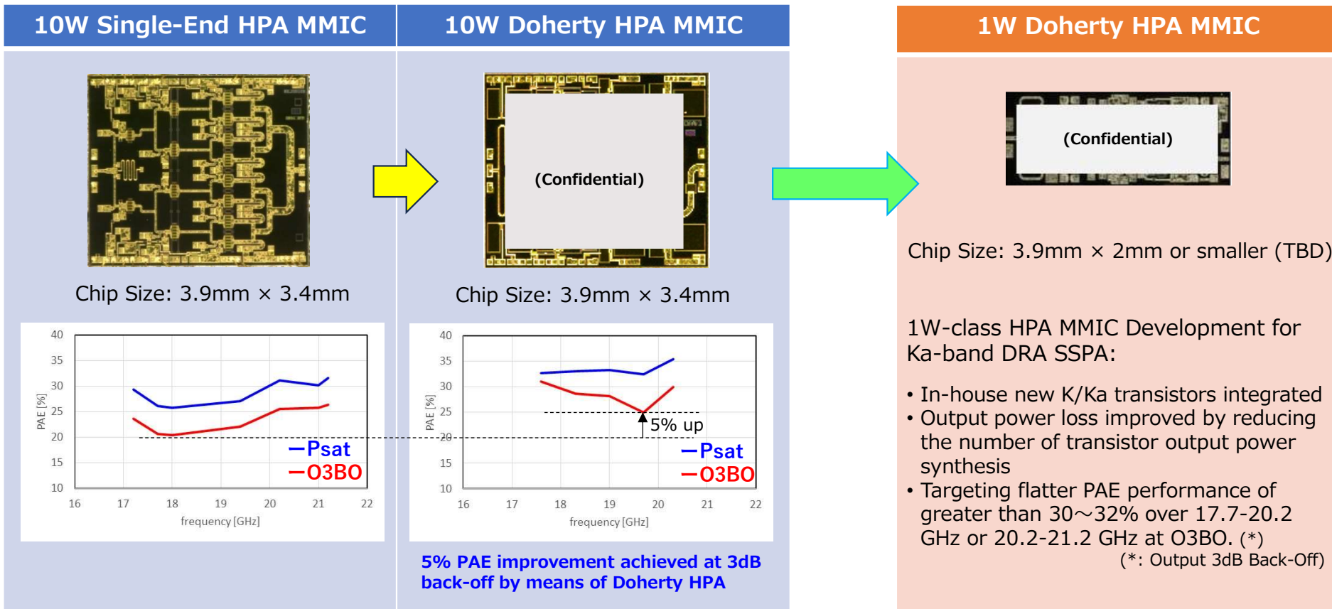
New HPA MMIC Design (1W-class)
